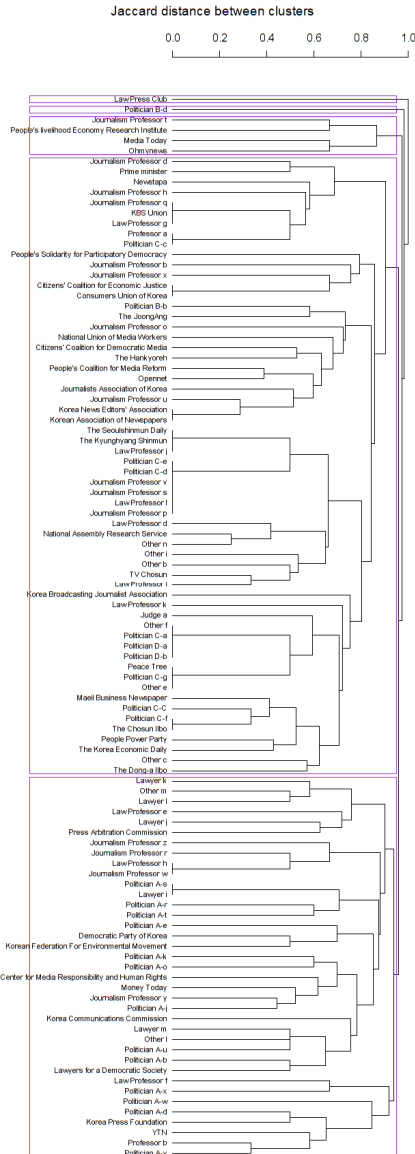
Figure 3. Result of hierarchical clustering in the 2 nd period
