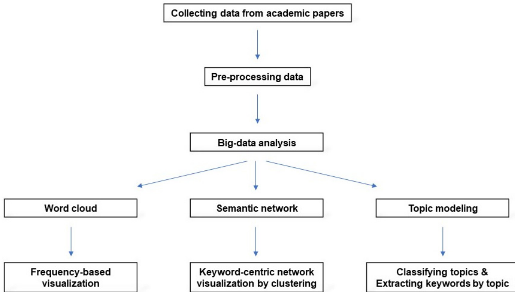
Figure 1. Research Process
